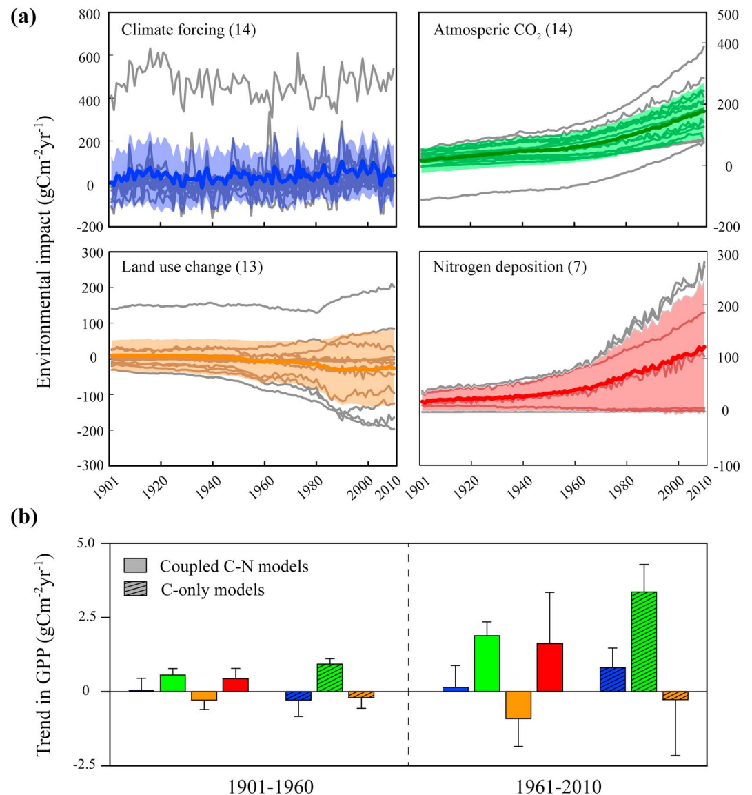
Figure 5. (a) The impact of climate forcing, atmospheric CO 2 , land-use change and nitrogen deposition on the dynamics of GPP in the East Asian monsoon region between 1901 and 2010. The gray lines are results from individual models, and the bold colored lines and the shaded areas are respectively the calculated average and standard deviation among models. The number of models is shown in parentheses. (b) Trends in GPP driven by climate forcing, atmospheric CO 2 , land-use change and nitrogen deposition using segmented linear regression breaking at the sixtieth. Error bars show the standard deviation among models.
