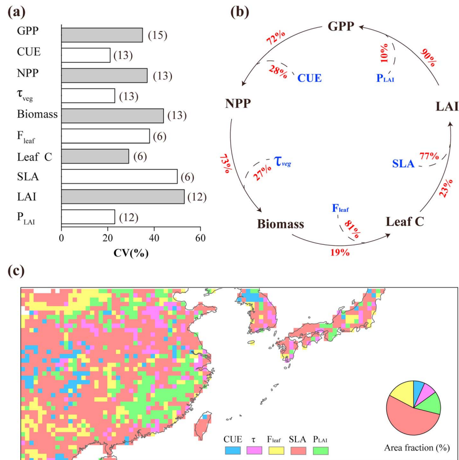
Figure 4. (a) Intermodel variability (coefficient of variation: CV = 100 \times SD/mean ) of key carbon processes and vegetation functional properties. Numbers behind the bars indicate the number of models provide outputs for the carbon processes and vegetation functional properties. (b) Relative importance of key carbon processes and the associated vegetation functional properties in controlling model performance on GPP. (c) Contributions of the five vegetation functional properties in driving GPP.
