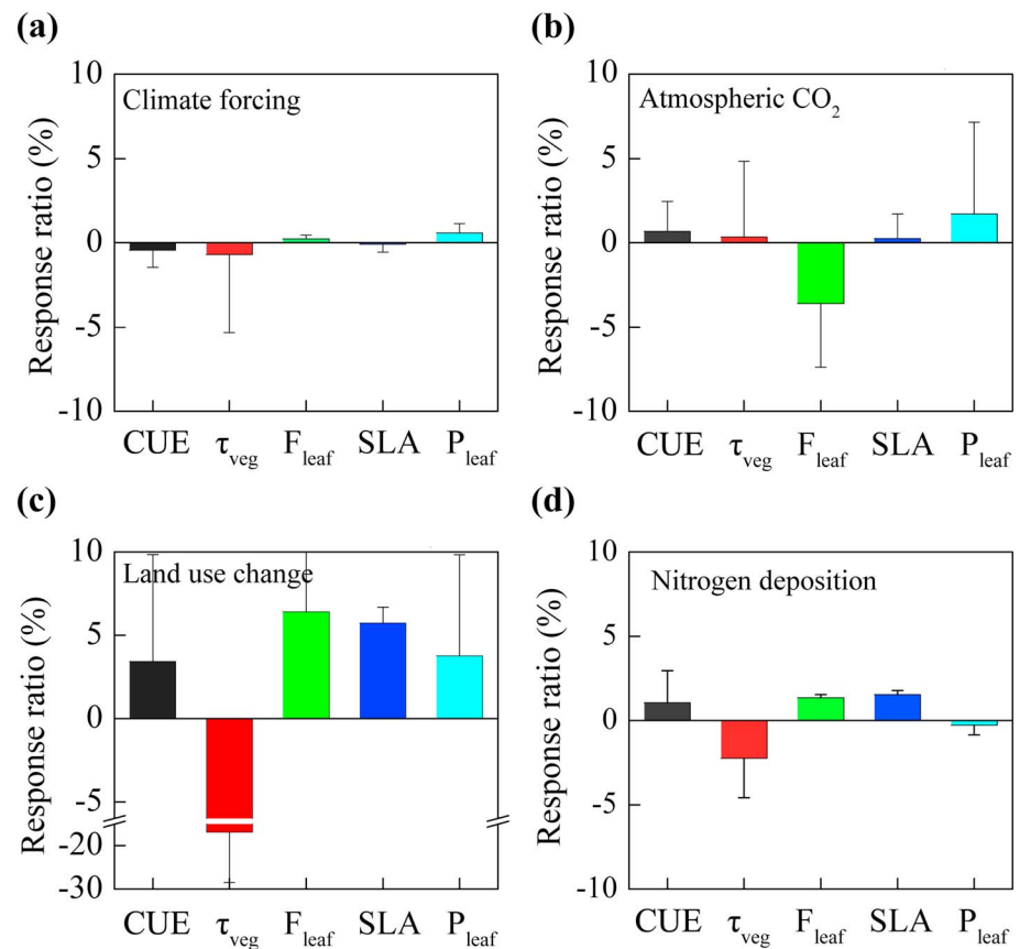
Figure 6. The simulated response ratios of vegetation functional properties to climate forcing (a), atmospheric CO 2 (b), land-use change (c) and nitrogen deposition (d). Error bars show the standard deviation of response ratios among models.
