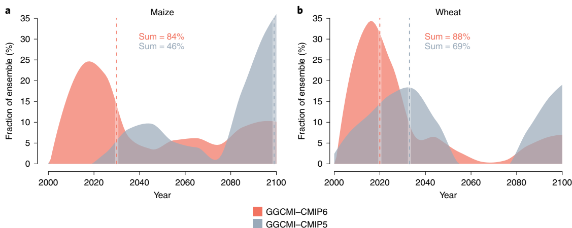
Fig. 4 | Shift towards earlier and more pronounced climate impact emergence. a,b , Density plots of individual TCIE estimates across the GCM × GGCM ensemble under SSP585 are shown for global maize productivity ( a ; negative TCIE) and global wheat productivity ( b ; positive TCIE). Histogram counts are smoothed with a locally weighted fit (LOESS; span, 0.5) and shown as the fraction of the respective ensemble size. The GGCM-6 ensemble includes 12 crop models, GGCM-5 includes seven crop models; both comprise five GCMs. The total ensemble fraction that shows TCIE by 2099 is indicated by ‘Sum’. The ensemble median TCIE is highlighted with vertical dashed lines. See Supplementary Fig. 4 for soybean and rice.
