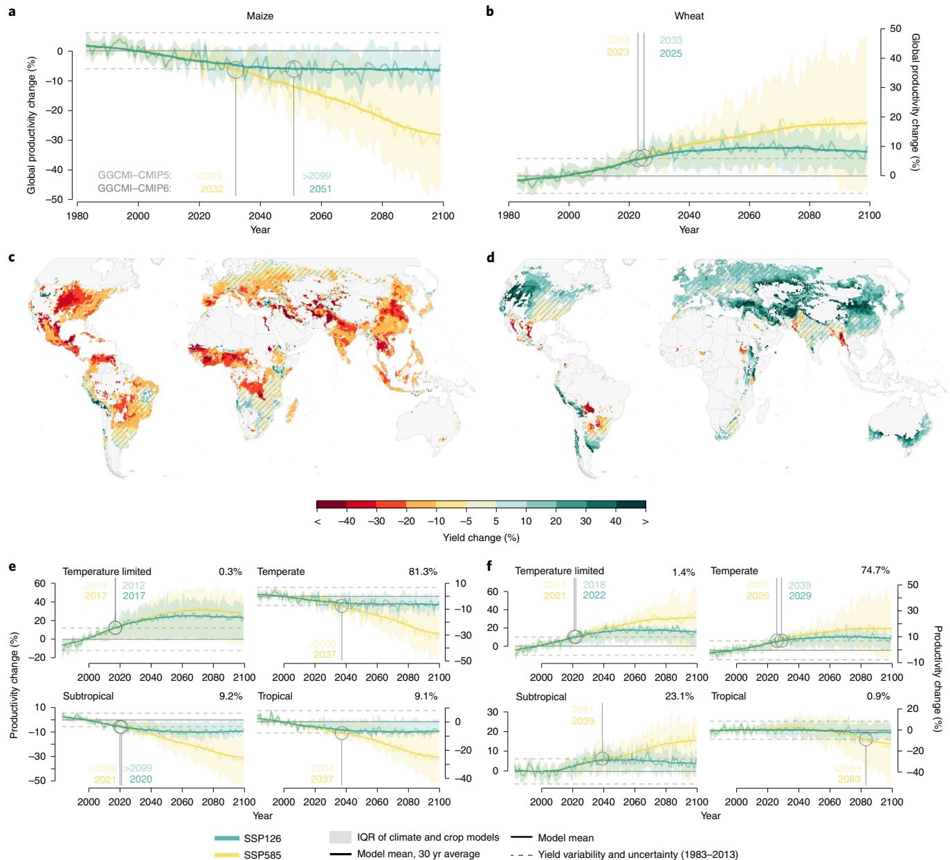
Fig. 3 | Projections of global crop productivity for the twenty-first century. a, b , Productivity time series for maize ( a ) and wheat ( b ) shown as relative changes to the 1983–2013 reference period under SSP126 (green) and SSP585 (yellow). Shaded ranges illustrate the IQR of all climate–crop model combinations (5 GCMs \times 12 GCMs). The solid line shows the median response (and a 25 yr moving average). Horizontal dashed lines mark the standard deviation of historical yield variability and model uncertainty (that is, ‘noise’ from individual climate–crop model combinations) and open circles highlight the TCIE, the year in which the smoothed climate change response emerges from the noise. For context, the TCIE calculated from GC5 (ref. 7) simulations is indicated in lighter shades above the TCIE based on GC6 (>2099 if no TCIE occurs by 2099). c, d , Maps showing median yield changes (2069–2099) for maize ( c ) and wheat ( d ) under SSP585 across climate and crop models for current growing regions (>10 ha). Hatching indicates areas where <70% of the climate–crop model combinations agree on the sign of impact. e, f , Regional productivity time series for maize ( e ) and wheat ( f ) similar to a , but stratified for the four major Koeppen–Geiger climate zones (temperature limited, temperate/humid, subtropical and tropical). The percentage of the total global production contributed by each zone is indicated in the top right corner of the insets. All data are shown for the default [\text{CO}_2] (see Supplementary Fig. 3 for all four crops).
