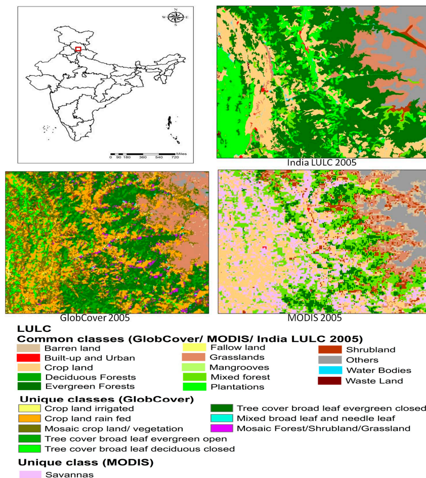
Figure 11. Comparison of resolution of LULC 2005 India product with MODIS Land Product and GlobCover—2005.
