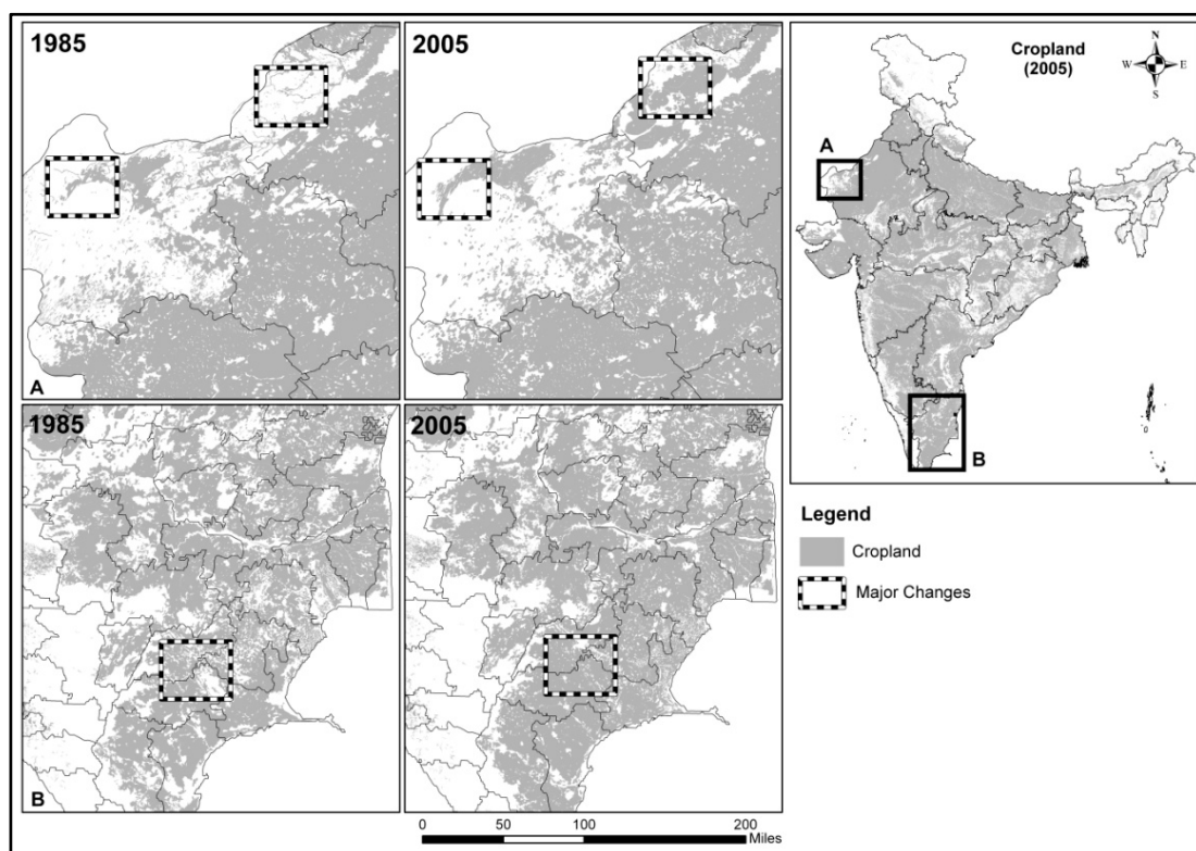
Figure 7. Increase in crop land during 1985 to 2005 in western India and east coast of south India.
