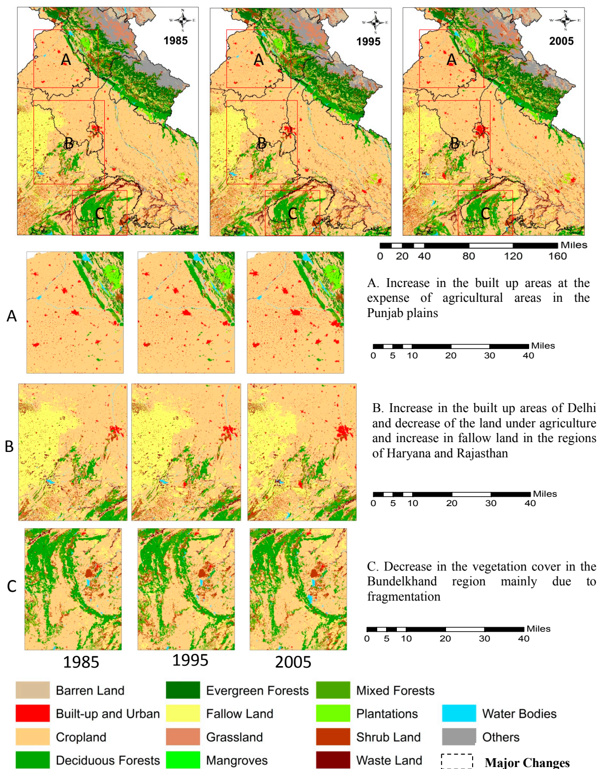
Figure 3. Land-use and land-cover changes in north western India over two decades (1985–2005). (A). Increase in the built up areas at the expense of agricultural areas in the Punjab plains. (B). Increase in the built up areas of Delhi and decrease of the land under agriculture and increase in fallow land in the regions of Haryana and Rajasthan. (C). Decrease in the vegetation cover in the Bundelkhand region mainly due to fragmentation.
