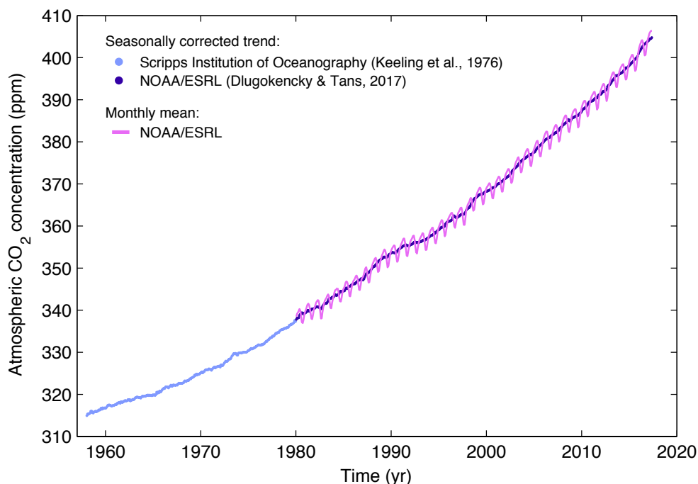
Figure 1. Surface average atmospheric CO 2 concentration, deseasonalised (ppm). The 1980-2017 monthly data are from NOAA/ESRL (Dlugokencky and Tans, 2017) and are based on an average of direct atmospheric CO 2 measurements from multiple stations in the marine boundary layer (Masarie and Tans, 1995). The 1958-1979 monthly data are from the Scripps Institution of Oceanography, based on an average of direct atmospheric CO 2 measurements from the Mauna Loa and South Pole stations (Keeling et al., 1976). To take into account the difference of mean CO 2 between the NOAA/ESRL and the Scripps station networks used here, the Scripps surface average (from two stations) was harmonised to match the NOAA/ESRL surface average (from multiple stations) by adding the mean difference of 0.542 ppm, calculated here from overlapping data during 1980-2012. The mean seasonal cycle is also shown from 1980 (in pink).
